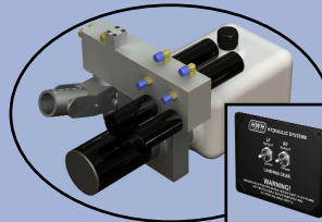
Hand /electric pump with remote operating panel
