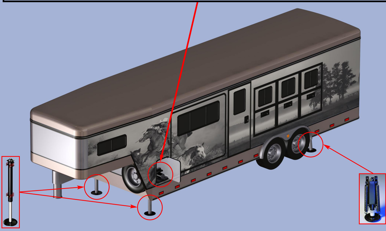
Hand pump with hydraulic switches (no electric power is required)
